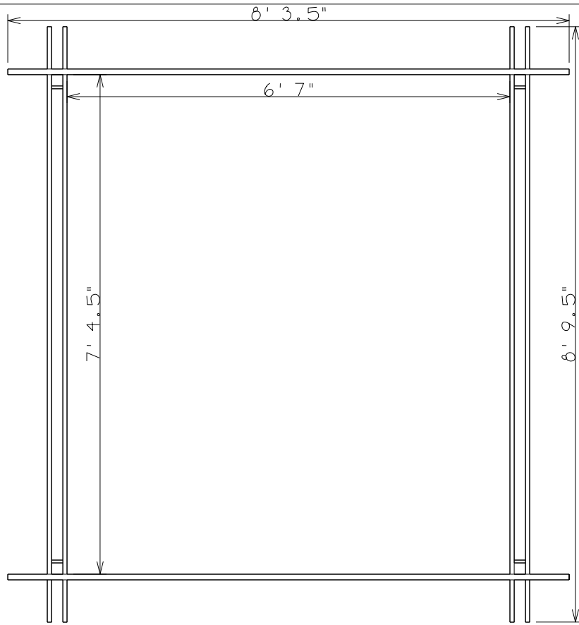
PLAN/TOP VIEW
